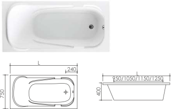
FC-302 SIZE: 1800X750X400MM 1600X750X400MM 1700X750X400 MM 1500X750X400MM 1) Acrylic built in bathtub 2) Overflow 3) Drainage
