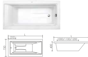
FC-313B SIZE: 1700X750X400MM 1600X750X400MM 1500X750X400MM 1) Acrylic built in bathtub 2) overflow 3) drainage
