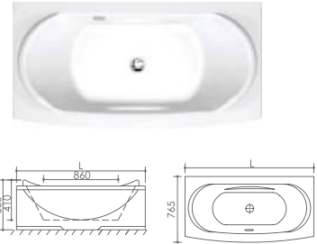
FC-315A SIZE: 1700X765X580MM 1600X765X580 MM 1500X765X580MM 1) Soaking acrylic bathtub 2) Support- Stainless steel frame 3) Cold & hot faucet,handshower,water in 4) Overflow & Drainage 5) Available version: left or right
