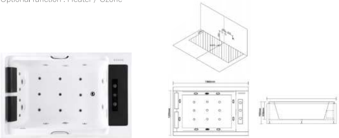
FC-2662HT SIZE:1860X1220X700MM 1) Whirlpool massage 2) Surrounding water fall 3) LED micro bottom massage jet 4) Touch control panel 5) Electric lift taps and handshower 6) Automatic draiange 7) water intake 8) 3 sides panel Optional function : Heater / Ozone
