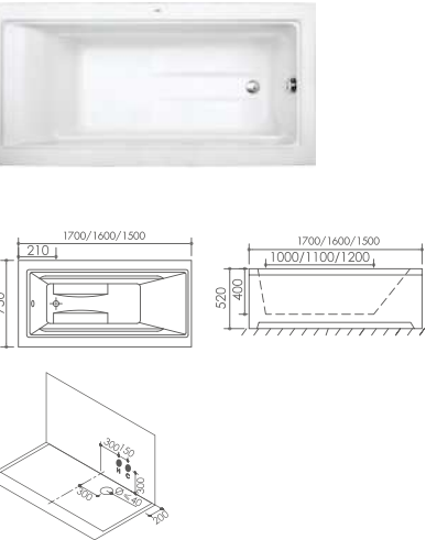
FC-313A SIZE: 1700X750X520MM 1600X750X520MM 1500X750X520MM 1) Soaking acrylic bathtub 2) Support- Stainless steel frame 3) Cold & hot water faucet,handshower,water in 4) Overflow & Drainage 5) Available version: left or right
