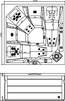
FC-SP403 ECO 2000X2000X900MM
