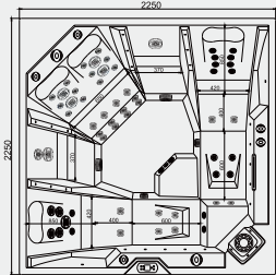
FC-SP404 ECO 2250X2250X900MM
