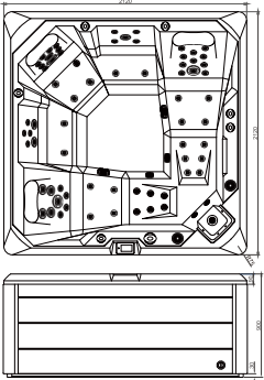
FC-SP701 ECO Extreme 2120X2120X900MM
