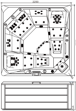
FC-SP703 ECO Extreme 2250X2250X900MM
