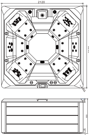
FC-SP702 ECO Extreme 2120X2120X900MM
