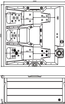
FC-SP402 ECO 2000X2000X900MM
