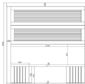
CUBE X3: 2250 x 2250 x 2370 mm
